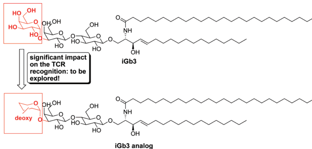
FIGURE 1. The design of the iGb3 analogues for the SAR study.
