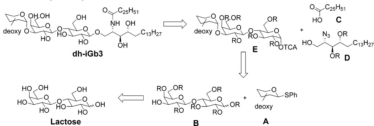
FIGURE 1. The design of the iGb3 analogues for the SAR study.
