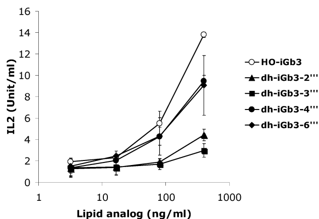
FIGURE 2. Activation of NKT cells with iGb3 analogues. (Data were the average of three independent experiments and analyzed by the SPSS data program. An independent-sample t -test was used to measure the statistic significance of the differences between HO-iGb3 and each deoxy-iGb3 analogue at data points of 400 ng/mL. For the difference between 2'''-dh-iGb3 and HO-iGb3, as well as the difference between 3'''-dh-iGb3 and HO-iGb3, the P value is lower than 0.001. For the difference between 4'''-dh-iGb3 and HO-iGb3, as well as the difference between 6'''-dh-iGb3 and HO-iGb3, the P value is lower than 0.05.)
